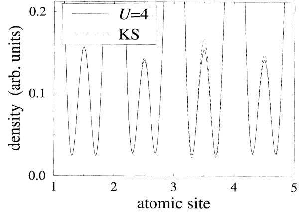
FIG. 1. Electron density of the eight-site Hubbard chain ( U = 4 ) together with that of the Kohn-Sham system that reproduces it as closely as possible (KS), visualized by assuming a particular form of orbitals (see the text). There is good agreement at the ends of the chain (site 1), but increasing deviation towards the center (site 5). The deviation illustrates the fact that the density of the interacting system is not noninteracting v representable.
