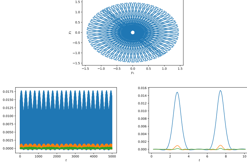
FIGURE 1. Numerical experiment with the multistep scheme (4.1) with A_2 = \text{diag}(0.85, 1.25) , A_1 = I - 4A_2 , U(y) = \exp(-\frac{1}{2}(y_1^2 + y_2^2)) and time-step h = 0.1 . The multistep formula was initialised at times 0, h, 2h, 3h by integrating the order 4 modified equation using very fine Euler-steps starting from the initial value (y_{\text{init}}, \dot{y}_{\text{init}}) = ((1, -1), (0.1, -0.2)) . The figure at the top shows a trajectory up to time t = 500 , which looks like an orbit in a completely integrable system. The figures below show an evaluation along the trajectory of H - H((y_{\text{init}}, \dot{y}_{\text{init}})) (blue) as well as H_{\text{mod}}^{[2]} - H_{\text{mod}}^{[2]}((y_{\text{init}}, \dot{y}_{\text{init}})) (orange) and H_{\text{mod}}^{[4]} - H_{\text{mod}}^{[4]}((y_{\text{init}}, \dot{y}_{\text{init}})) (green) up to time t = 5000 and t = 10 , respectively. We see oscillatory energy error behaviour.
