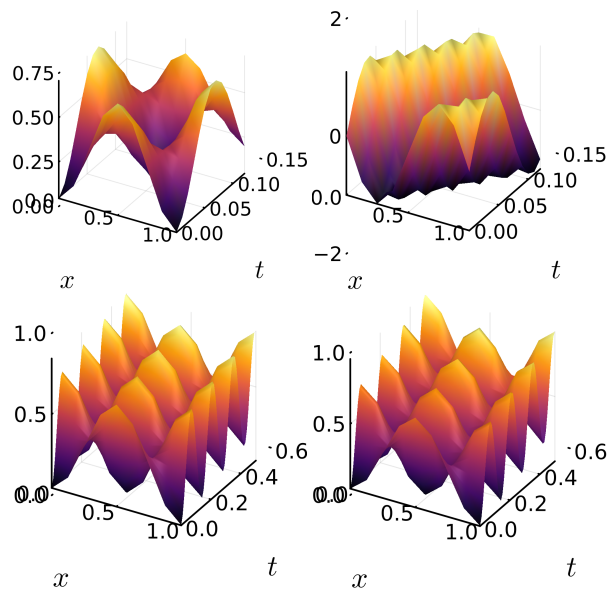
FIG. 13. Learned discrete Schrödinger equation. Top left: Sample of solution in training data (real part). Top right: Learned model reproduces travelling wave when initialised from exact travelling wave data (compare to left of Fig. 7). Bottom: Extrapolation of the solution with true discrete Lagrangian (left) and with the learned discrete Lagrangian (right) (error 0.01 in infinity norm).
